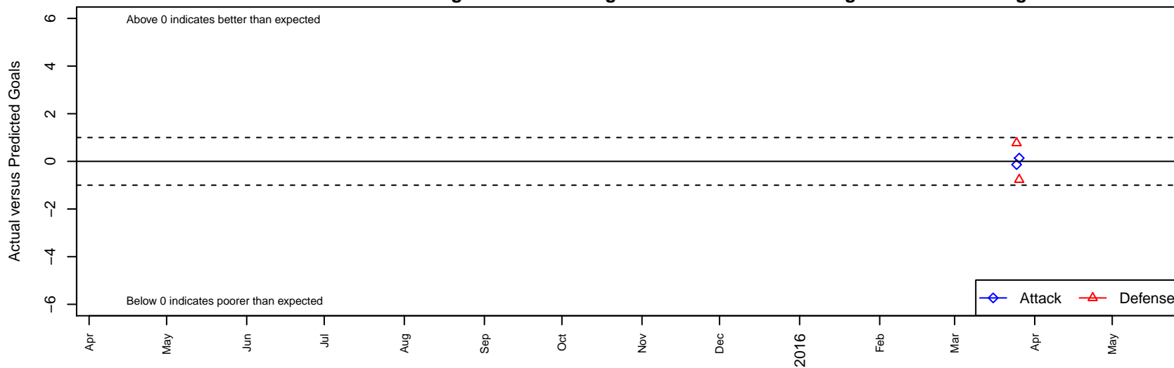
Victoria SC 2000G Dots are actual minus expected GF (blue circles) and GA (red triangles). Blue line is smoothed change in attack strength. Red is smoothed change in defense strength.
